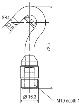
B-1 Small Hook (59g)
