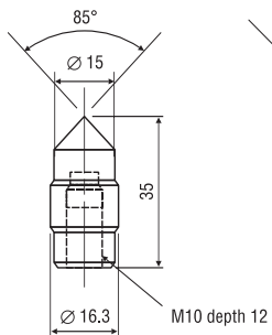
B-4 Chisel Tip (38g)
