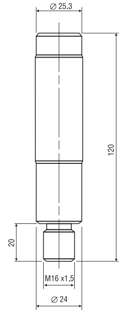
B-7 Handle (102g)
