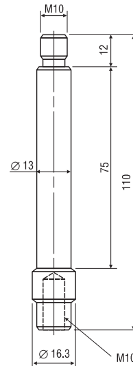
B-6 Extension Shaft (102g)
