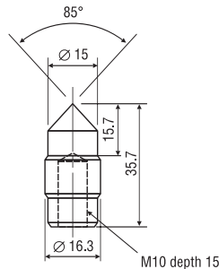
B-3 Conical Tip (33g)
