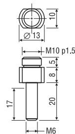
B-8 Mounting Bolts
