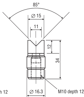
B-5 Notched Tip (38g)
